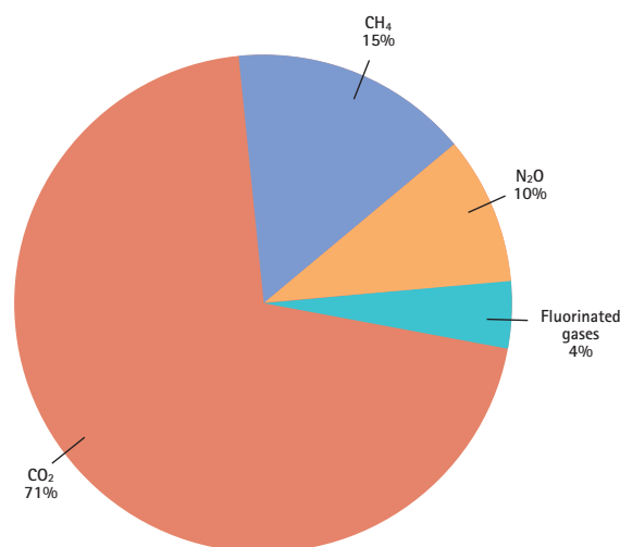
Figure 2.3.2a. Distribution of emissions of greenhouse gases by gas in 2003
