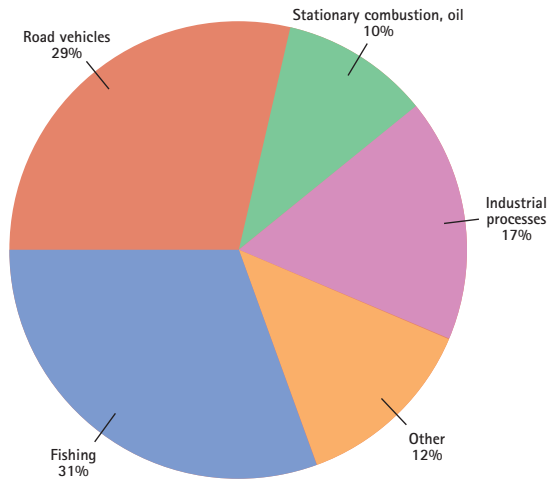
Figure 2.3.2c. Distribution of CO 2 emissions by source in 2003
