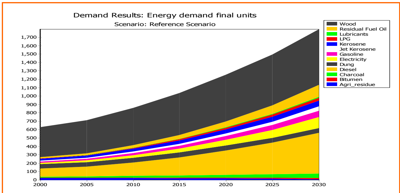
Figure 4.7: Total Projected Energy Demand by Type of Fuel- Reference Scenario (ktOE), (Source: NGHGMTWG, 2009)
