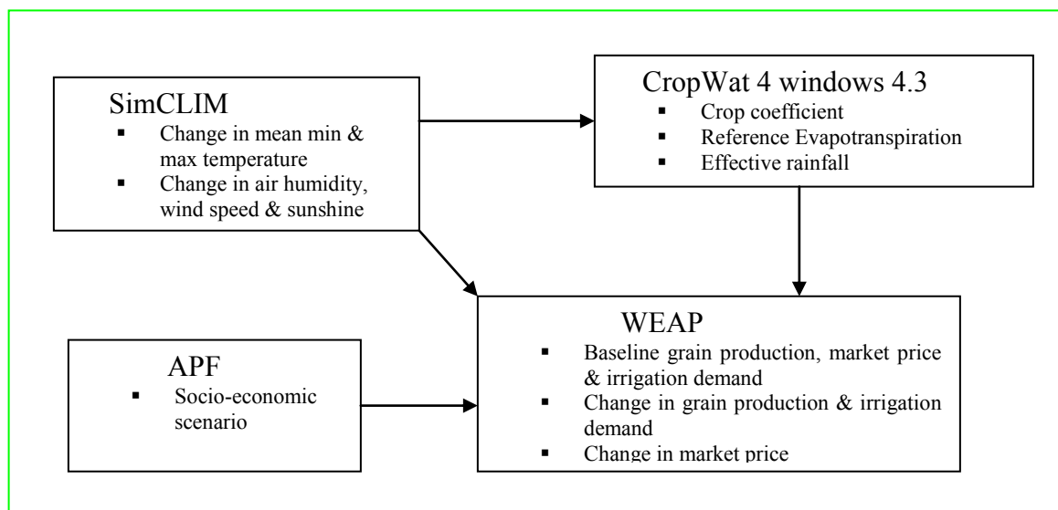
Figure 5.29: Conceptual Models Linkage for Crop Impact Assessment in Mereb-Gash Basin
